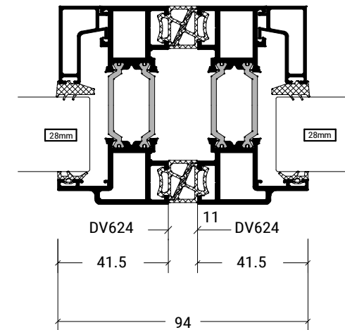
Stile cross-section
