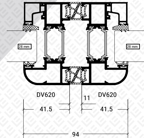
Stile cross-section
