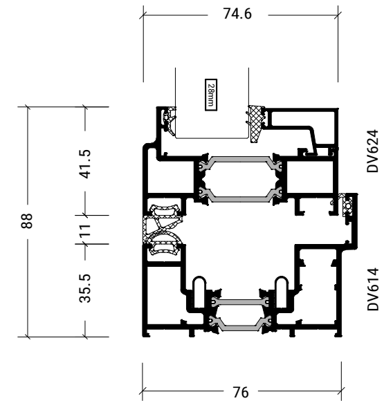
Profile section
