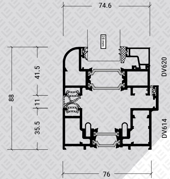
Profile section
